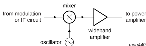
Fig 5. Application as driver amplifier.
